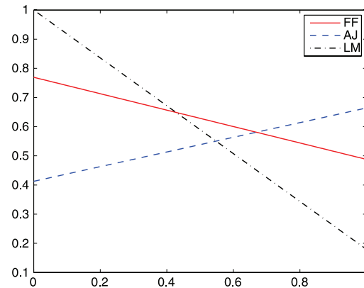
Fig. 3. Mean of weighted averages of sensitivity and specificity for FF, AJ, and LM tests over 1000 simulations when \Delta = 1 min and a_n = 30 . The x -axis represents the weight for sensitivity. The data are generated from model (25) with \lambda = 12 \times 21 .
