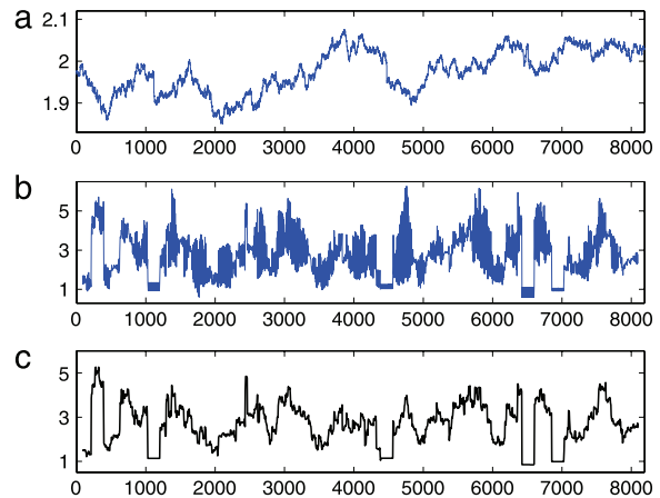
Fig. 2. Test statistics \tilde{S}(p, K)_t and \hat{S}(p, K)_{1,t} , with p = 4 and K = 2 as processes of time. The price process X_t is generated from model (25), with \Delta = 1 min and J_s = 0.05 . There are 4 jumps in total, which are located at time points 1115, 4474, 6512, and 6941. (a) X_t in a one-month period; (b) \tilde{S}(p, K)_t with local window size a_n = 90 ; (c) \tilde{S}(p, K)_t with local window size a_n = 90 .
