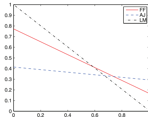
Fig. 4. Mean of weighted averages of sensitivity and specificity for FF, AJ, and LM tests over 1000 simulations when \Delta = 3 min and a_n = 30 . The x -axis represents the weight for sensitivity. The data are generated from model (25) with \lambda = 12 \times 21 .
