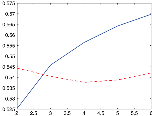
Fig. 1. Plot of M(p, K)/M^*(p, K) against K for p = 4 (solid curve) and p = 5 (dashed curve).
