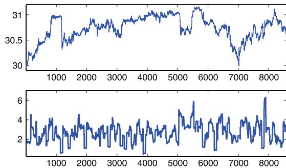
Fig. 5. Top panel: stock price data of Microsoft Corporation from May 1, 2007 to May 31, 2007 with 1-min frequency. Bottom panel: \tilde{S}(p, K)_t as a process of time with 2a_n = 78 .
